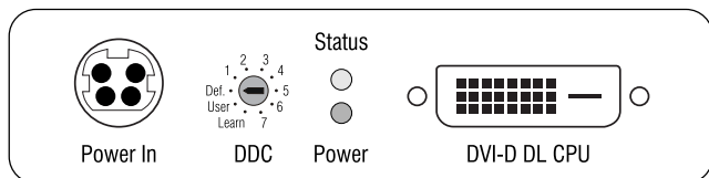
Figure 2: Back panel
