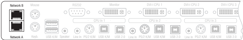
Figure 4: Interfaces to connect local networks
