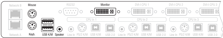
Figure 2: Interfaces to connect the console devices
