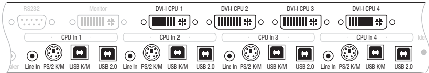
Figure 3: Interface to connect the computers
